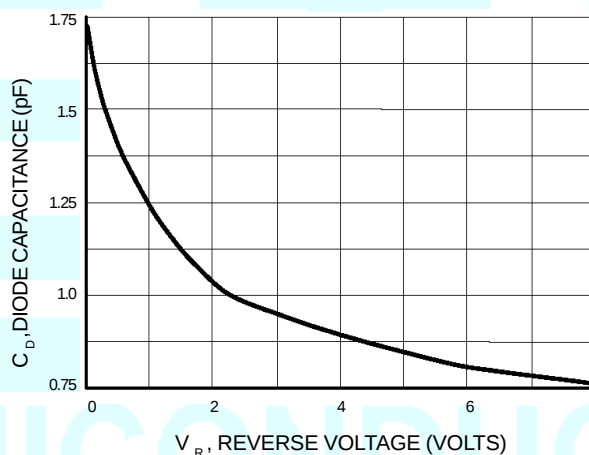
Figure 4. Capacitance
