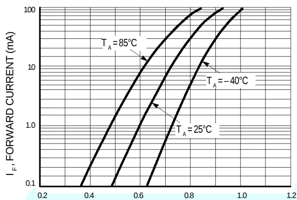
Figure 2. Forward Voltage
