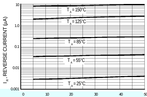
Figure 3. Leakage Current
