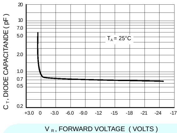
Figure 3. Diode Capacitance
