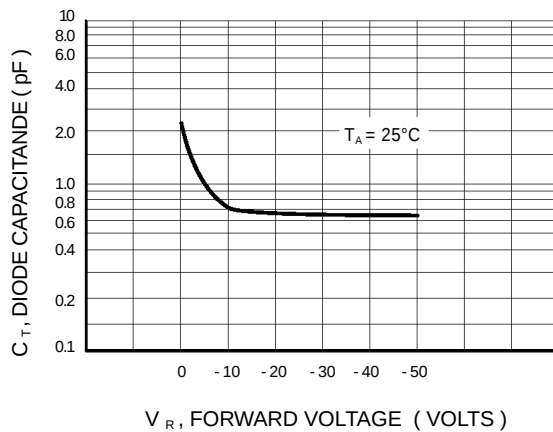
Figure 3. Diode Capacitance
