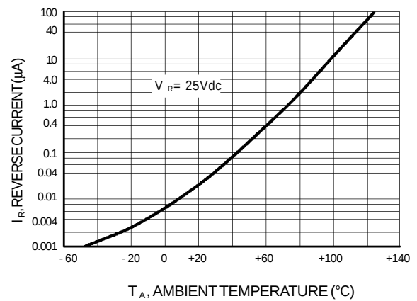
Figure 4. Leakage Current
