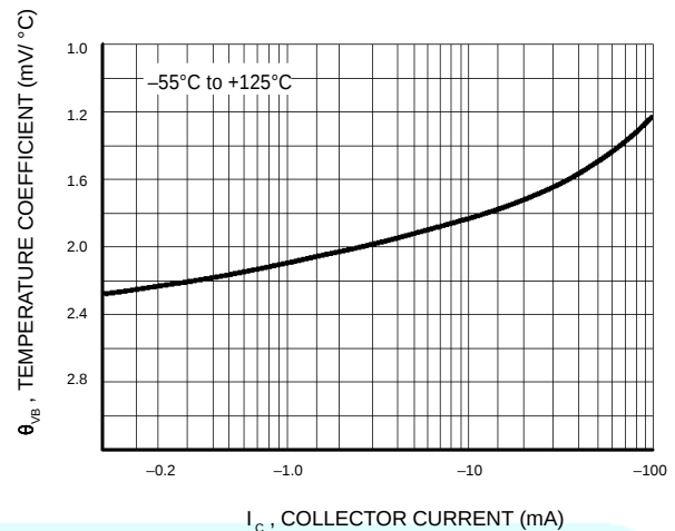
I_C , COLLECTOR CURRENT (mA) Figure 4. Base-Emitter Temperature Coefficient
