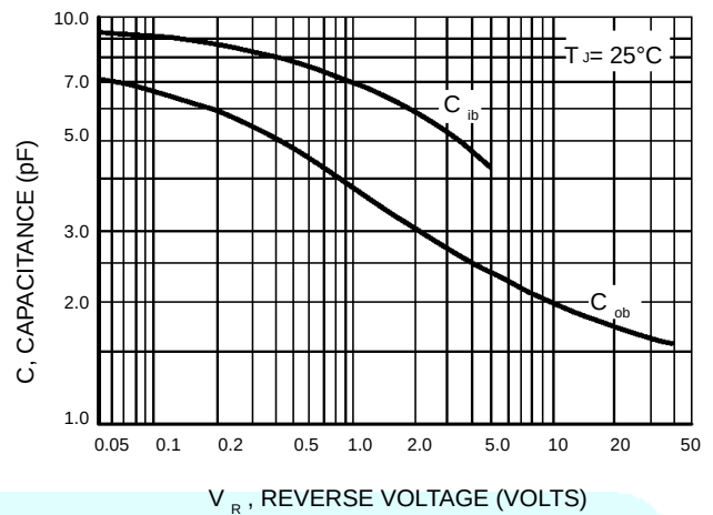
Figure 13. Capacitance
