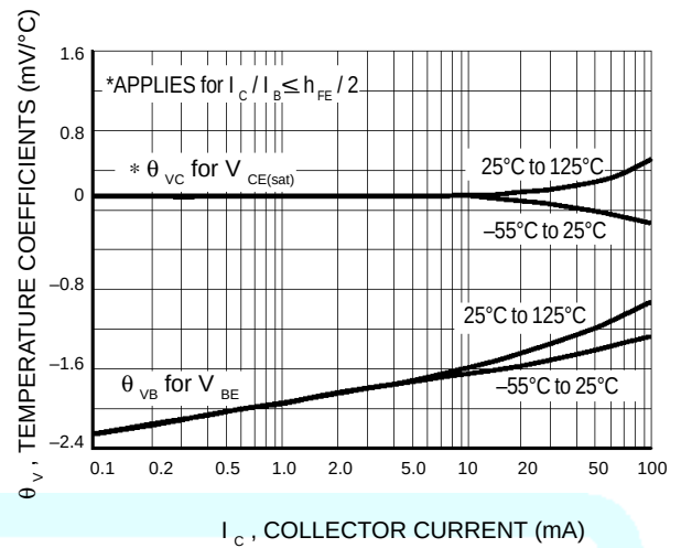
Figure 9. Temperature Coefficients
