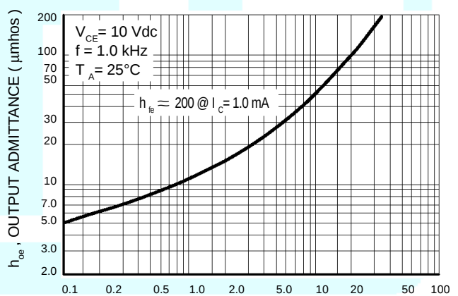
Figure 18. Output Admittance
