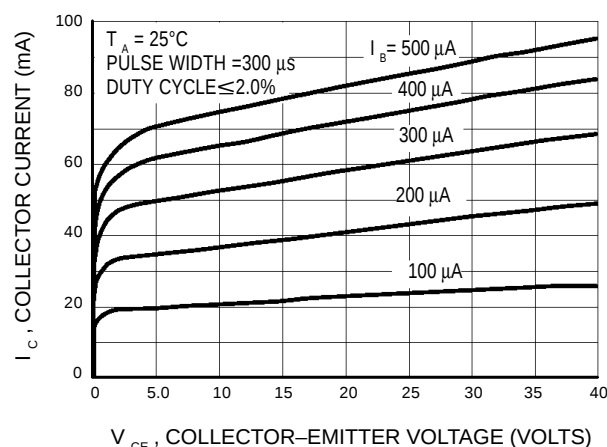
Figure 10. Collector Characteristics
