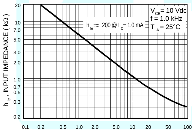
Figure 17. Input Impedance
