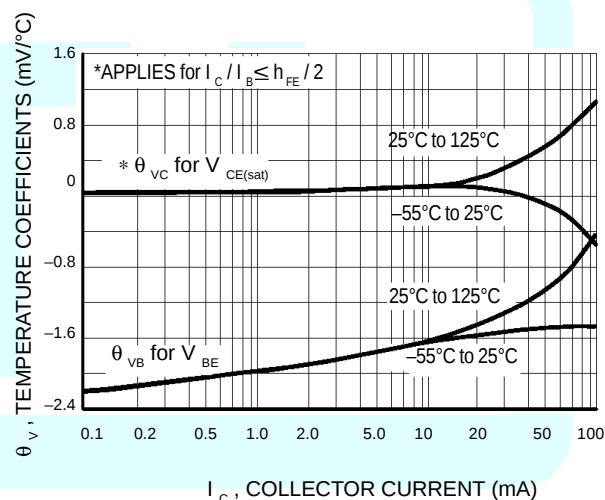
Figure 12. Temperature Coefficients
