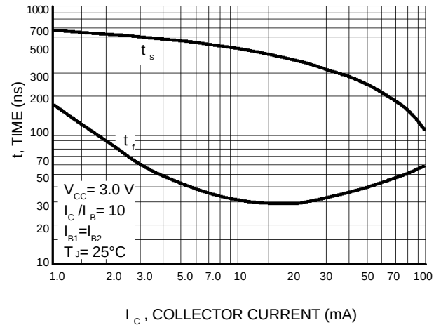
Figure 14. Turn-Off Time
