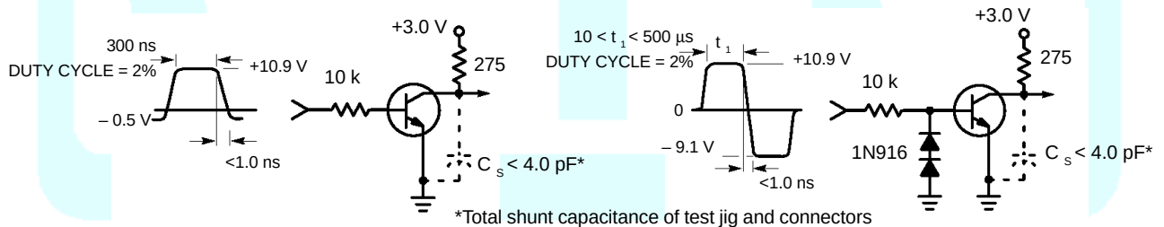
Figure 2. Turn-Off Time
