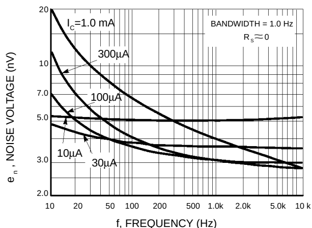
Figure 3. Noise Voltage
