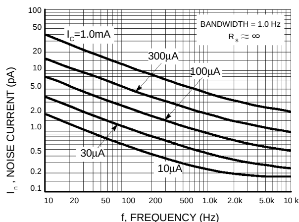
Figure 4. Noise Current
