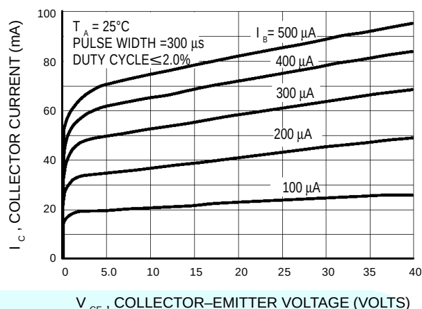
Figure 10. Collector Characteristics
