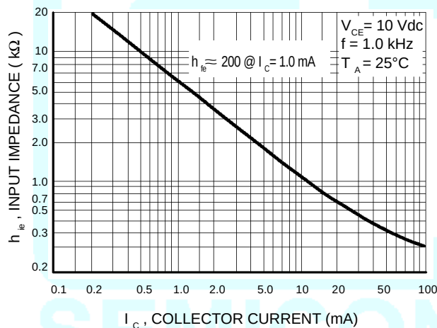
Figure 17. Input Impedance
