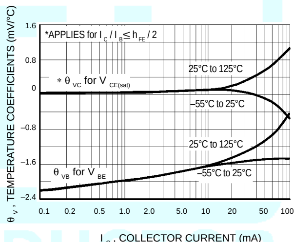
Figure 12. Temperature Coefficients
