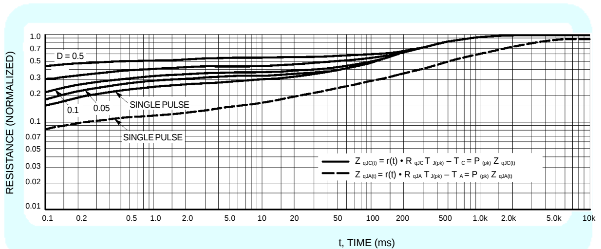
Figure 9. Thermal Response
