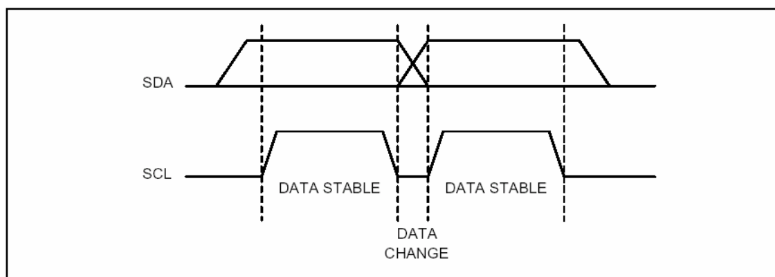
Figure 5. DATA VALIDITY
