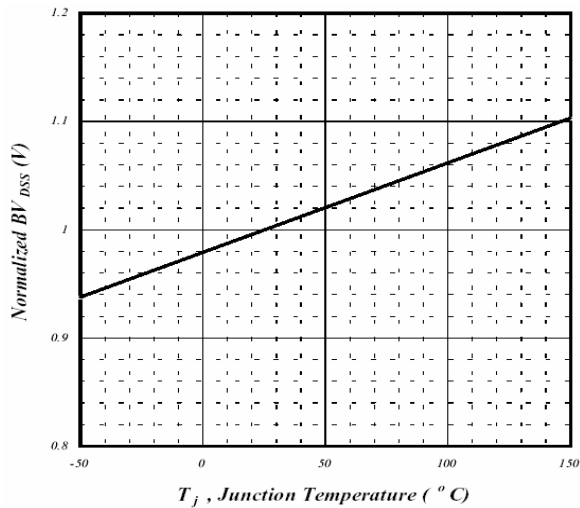
Fig 3. Normalized BV DS v.s. Junction Temperature
