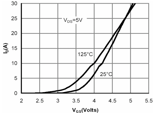
Fig 2. Transfer Characteristics
