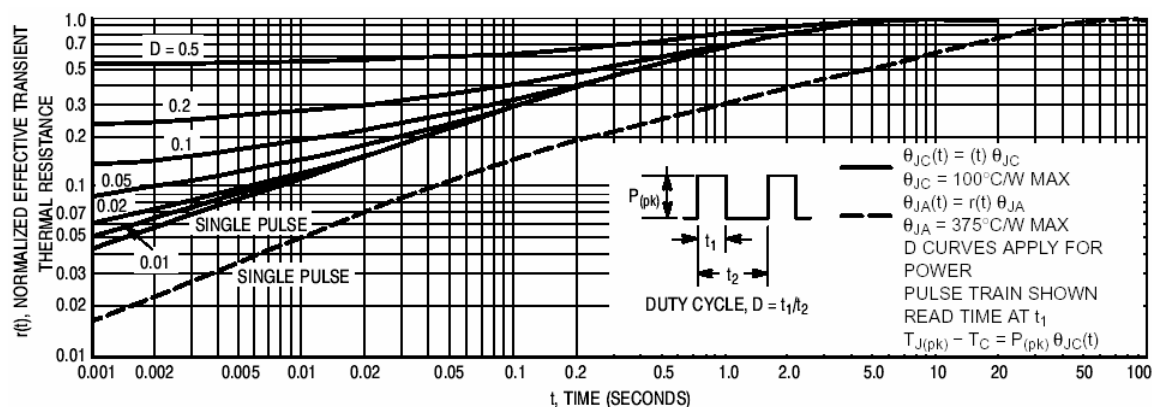
Fig 7. Thermal Response
